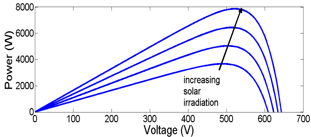
Figure 1- Power vs. Voltage graph of PV panel
