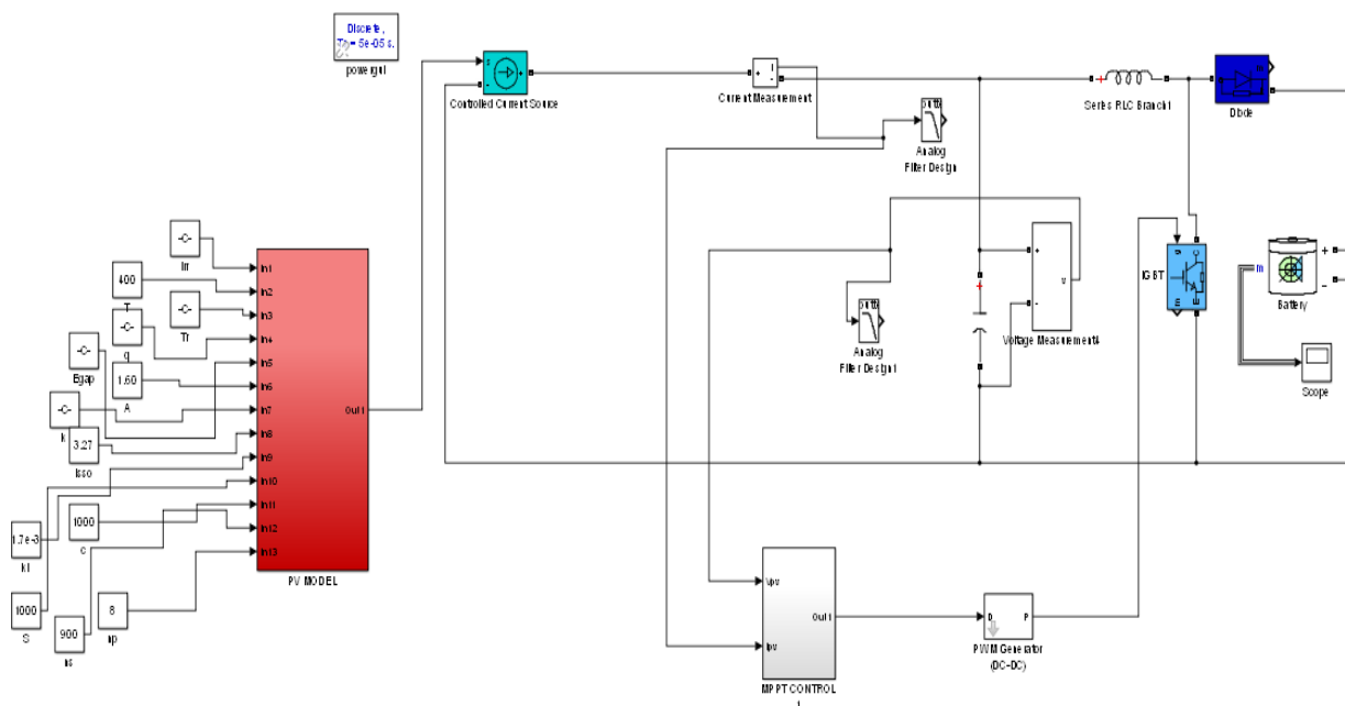
Figure 4 – The Simulation model of Stand Alone PV System with Battery Backup and MPPT control
